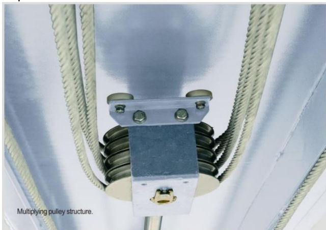
Multiplying pulley
